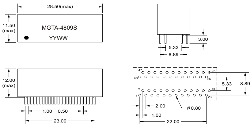
Dimensions: mm Unless otherwise specified, all tolerances are ±0.25
